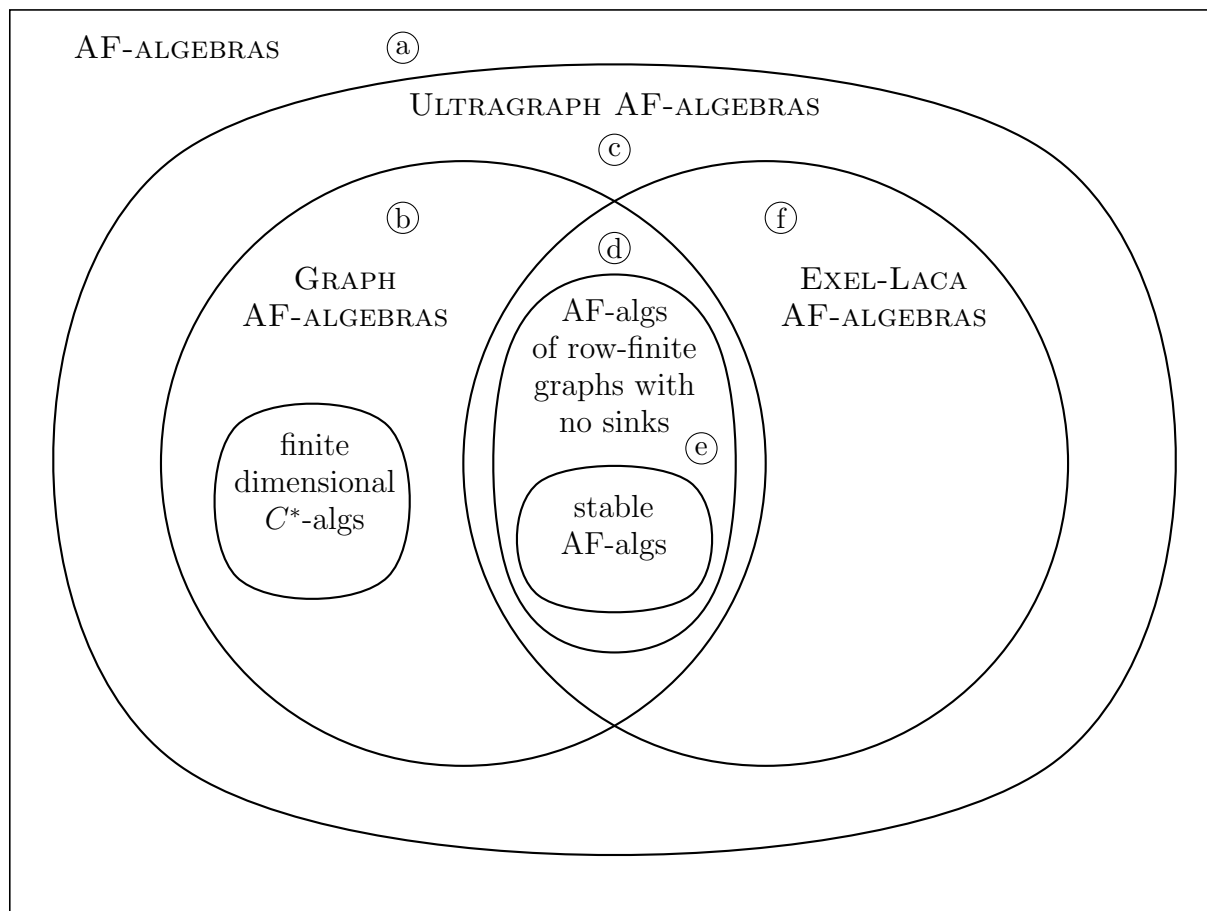
FIGURE 2. A Venn diagram summarizing AF-algebra containments
