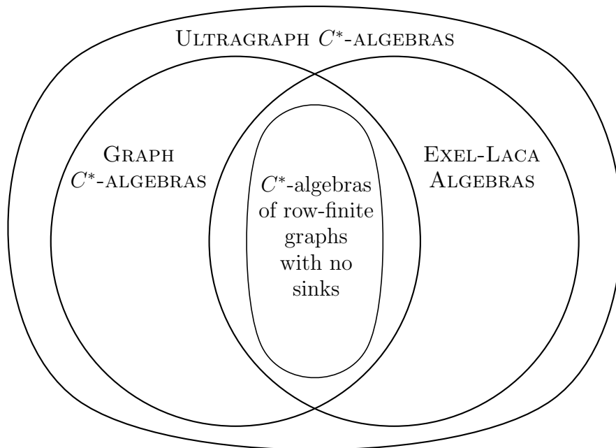
FIGURE 1. The relationship among graph C^* -algebras, Exel-Laca algebras, and ultragraph C^* -algebras
