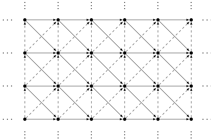
FIGURE 3. The skeleton of the 2-graph \mathcal{X} .
