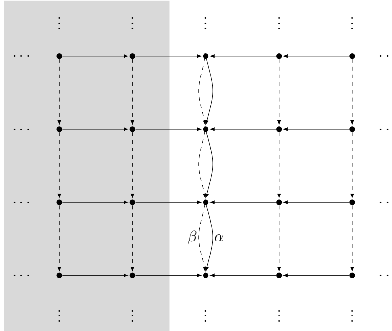
FIGURE 1. The skeleton of the 2-graph \mathcal{S} .
