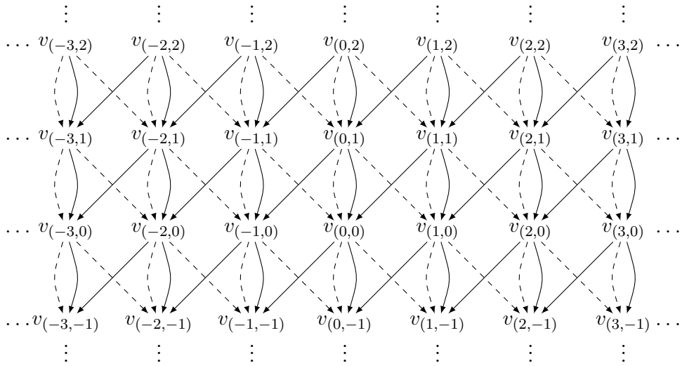
FIGURE 2. The common skeleton of the 2-graphs \Lambda_I and \Lambda_{II} .
