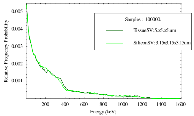
Figure 7: Geometry Case 2 (Example 1): Energy Deposition Spectra comparison of Silicon ( 3.15 \times 3.15 \times 3.15 \mu\text{m} ) and Tissue ( 5 \times 5 \times 5 \mu\text{m} ).
