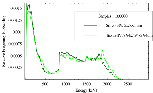
Figure 5: Geometry Case 1 (Example 2): Energy Deposition Spectra comparison of Silicon ( 5 \times 5 \times 5 \mu\text{m} ) and Tissue ( 7.9 \times 7.9 \times 7.9 \mu\text{m} ).
