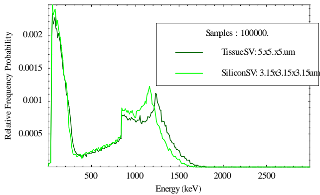
Figure 4: Geometry Case 1 (Example 1): Energy Deposition Spectra comparison of Silicon ( 3.15 \times 3.15 \times 3.15 \mu\text{m} ) and Tissue ( 5 \times 5 \times 5 \mu\text{m} ).
