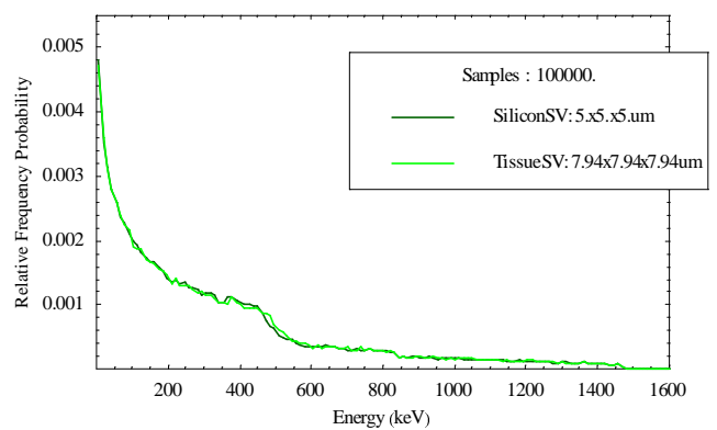
Figure 8: Geometry Case 2 (Example 2): Energy Deposition Spectra comparison of Silicon ( 5 \times 5 \times 5 \mu\text{m} ) and Tissue ( 7.9 \times 7.9 \times 7.9 \mu\text{m} ).
