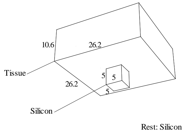
Figure 6: Geometry Case 2 - GV is a large tissue volume above a much smaller silicon/tissue SV
