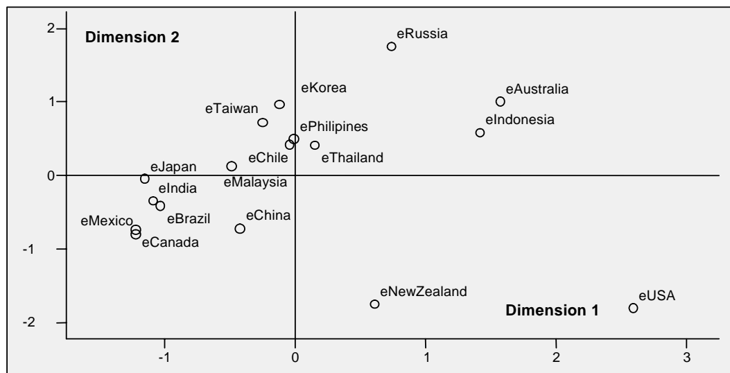
Figure 6 Scaling analysis: derived stimulus configuration
