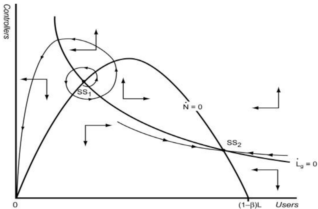
Figure 1: Phase-plane diagram with r > F'(0; (1-b)L)
